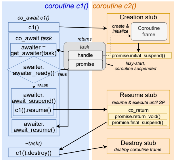
Figure 8: Coroutine lifetime (when a coroutine is co_await -ed from another coroutine, as in the program at Listing 2).
