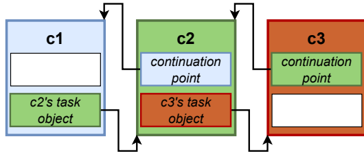
Figure 3: Internal objects that point to previous and next coroutine frames in a program with three nested coroutines.
