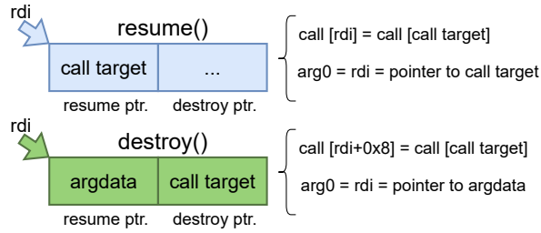
Figure 5: Hijacking of the call target and first argument via the resume and destroy pointers.
