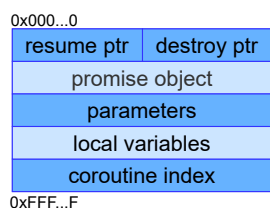
Figure 1: Coroutine frame structure in C++20.
