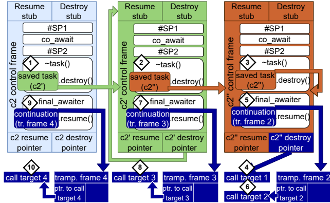
Figure 4: ICC attack on the program at Listing 2, showing how CFPs redirect the execution throughout the injected control and trampoline frames.
