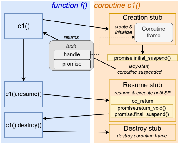
Figure 2: Coroutine lifetime (when executed from a function).
