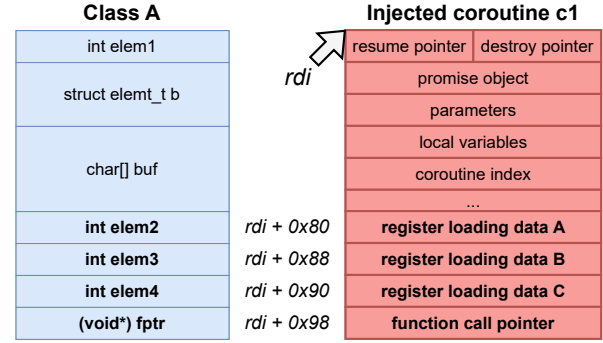
Figure 6: Use of a golden gadget at a member function to load arbitrary register values from an injected coroutine frame.
