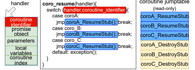
Figure 7: Proposed CFOP defense, moving vulnerable pointers to read-only memory, referenced by a coroutine identifier .
