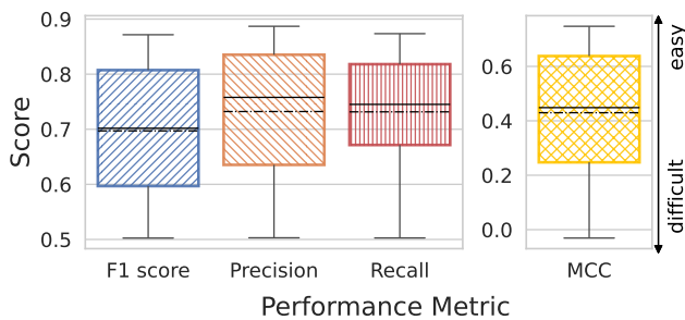
Figure 10: Evaluation using one unseen DGA family in the test set. While some DGA families have similarities with others and can still be detected, the general performance is degraded for unseen families. Any generalization claim does not hold for families with F1 score \leq 0.7 .
