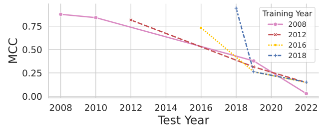
Figure 11: Evaluation by years, using DGArchive. The effects of training a model with data up to a year and testing it with future data. The training set includes samples up to the "training year", and the test set includes samples from the "test year".
