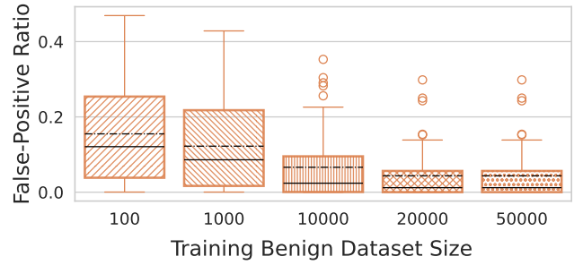
Figure 4: False-Positive Ratio on unseen Tranco samples, by the number of selected top- N samples. Each boxplot is constructed by training each DGA family individually against the selected top- N non-DGA samples and testing on 150k unseen Tranco samples. The dashed line is the average ratio, while the solid line is the median ratio across all families.
