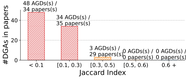
Figure 17: The Difficulty of the DGA per papers, using the Jaccard Index the non-DGA dataset (Tranco) and the DGA families. The count of unique DGAs in the experimental sections of related work, grouped by the Jaccard Index.
