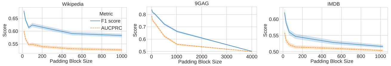
Figure 11: Performance when padding the flows against page fingerprinting. Left: Wikipedia. Middle: The 9GAG. Right: IMDB. We assume an advanced attacker who knows the padding strategy for each dataset and augments the training dataset.
