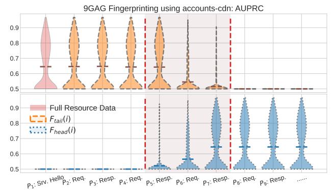
Figure 20: Critical Window Of Prediction Support Zoom-in For Single-flow Page Classification (AUPRC). Per-payload performance for each flow that carries important information is demonstrated on a flow from 9GAG. The benchmarks are done using 1000 labels from each dataset.
