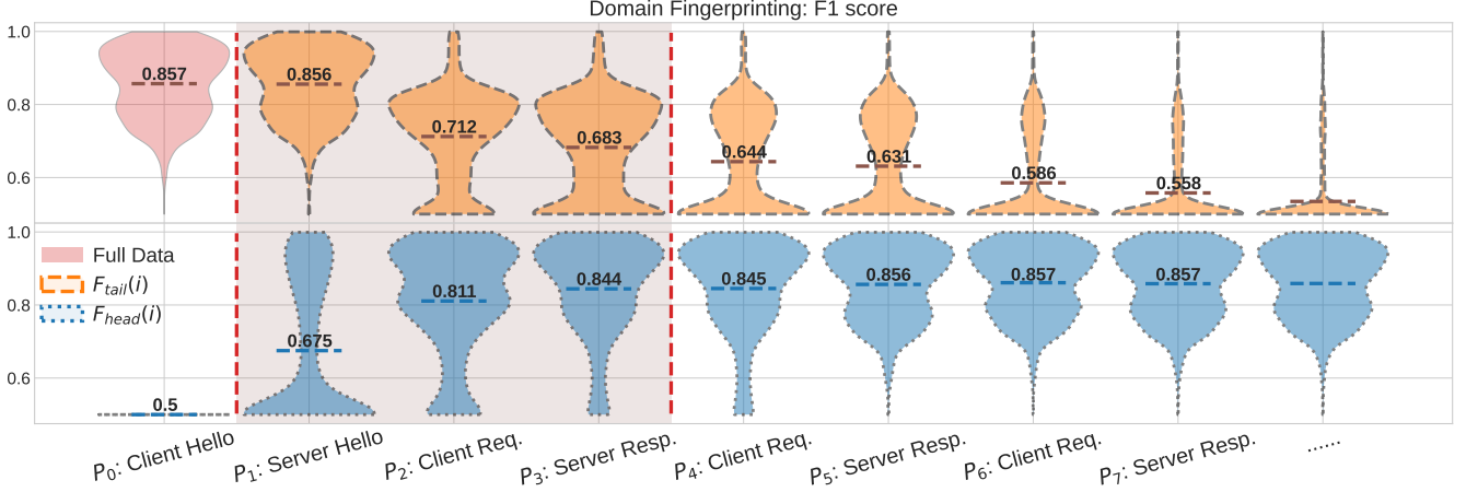
Figure 2: Detection of the Critical Window of prediction support for Domain fingerprinting (6472 domains) as violin plot. Each violin plot shows the distribution of F1 scores (y-axis) of all tested domains, differentiated by which HTTPS payloads are included (x-axis). We highlight two perspectives: a) Mask before P_i : At F_{tail}(i) , we classify only the payloads starting with index i (orange, dashed border, top) – i.e., the effect of excluding payloads P_0 - P_{i-1} . The upper lane also includes the performance on the entire flow (red, solid border, first on the left); and b) Mask after P_i : At F_{head}(i) , we consider only the first i payloads (blue, dotted border, bottom), i.e., the effects of including only payloads P_0 - P_i for fingerprinting. The dashed horizontal line is the mean of the scores of each violin next to the numerical value of it. The critical window for prediction support (Definition 3.1) is located between red dashed vertical bars and with a gray overlay.
