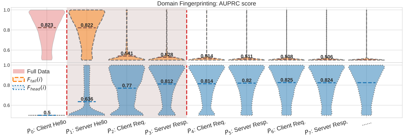
Figure 13: Detection of the Critical Window of prediction support for Domain fingerprinting (6472 domains) as violin plot. Each violin plot shows the distribution of AUPRC scores (y-axis) of all tested domains, differentiated by which HTTPS payloads are included (x-axis). The legend and representation have the same meaning as in Figure 2.
