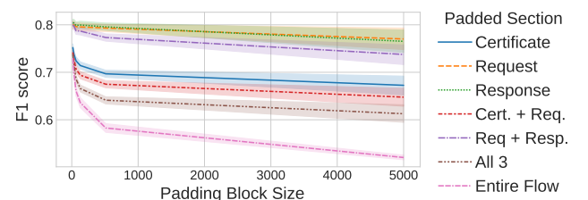
Figure 14: Attack performance by the size of the padding block (F1 score).
