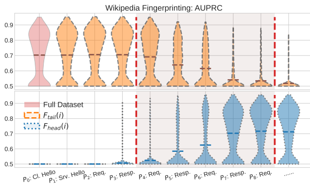
Figure 16: Critical Window Of Prediction Support for Page Detection on the Wikipedia dataset (AUPRC score).
