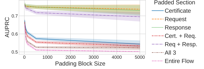
Figure 3: Domain fingerprinting performance by the size of the padding block, using the AUPRC metric. The critical window of prediction support is labeled using ‘All 3’: certificate, client request, and server response ( P_1 - P_3 ).
