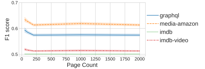
Figure 8: Page Detection on IMDB using a Single Flow. The flow imdb.com (green) offers less entropy than the api.graphql (blue) and media-amazon (orange) subdomains.
