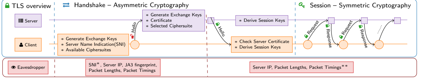
Figure 1: High-level overview of a TLS 1.3 session. The Client (orange) and Server (violet) agree on the session keys to secure subsequent HTTPS requests/responses. The Eavesdropper (red) indicates which information can be leaked from each phase. *SNI is assumed to be encrypted (ECH). **The Certificate is encrypted since TLS 1.3.
