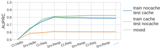
Figure 15: HTTP Caching impact on the Domain fingerprinting problem (AUPRC score). The scenarios are: (1) train on data without any HTTP caching example and test on data with HTTP(S) caching (blue line), (2) train on data with any HTTP(S) caching example and test on data without HTTP(S) caching (orange line), and (3) train on a mixture of data with and without caching and also test on an unseen mixture (green line).
