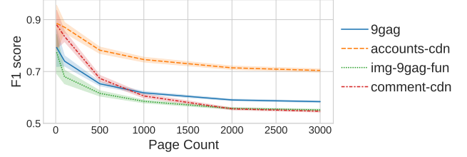
Figure 7: Page Detection on 9GAG using a Single Flow. The main flow 9gag.com (blue) leaks less information than the accounts-cdn (orange) subdomain.
