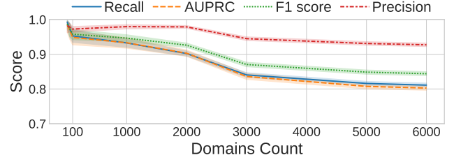
Figure 5: Domain detection performance by the number of distinct labels in the dataset. A model evaluated with fewer than 100 labels will report close to perfect scores. The performance decreases with the number of labels due to collisions in the certificate lengths, requests, and responses.
