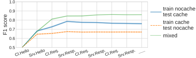
Figure 4: HTTP(S) Caching impact on the Domain fingerprinting problem. The scenarios are: (1) train without any HTTP(S) caching examples and test on caching samples only (blue solid line), (2) vice versa (orange dashed line), and (3) train and test on a mixture of data with/without caching samples (green dotted line).
